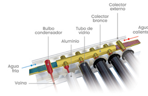
Despiece
